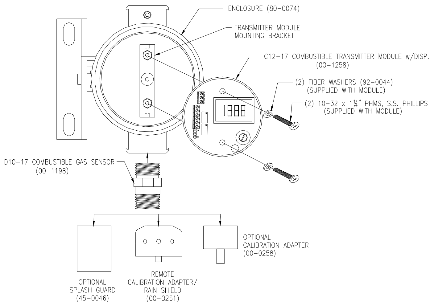
Figure 11 – Standard Combustible Transmitter Exploded View (ATI-0571)
