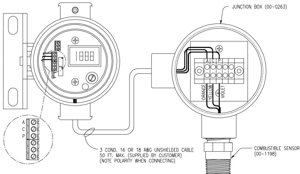
Figure 5: Dual Condulet Connections (ATI-0579)
