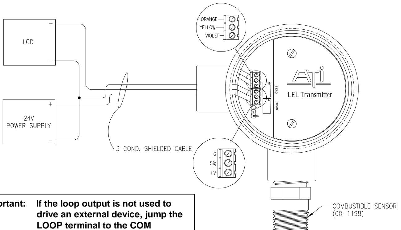
Figure 3: Transmitter customer connections (ATI-0237)
