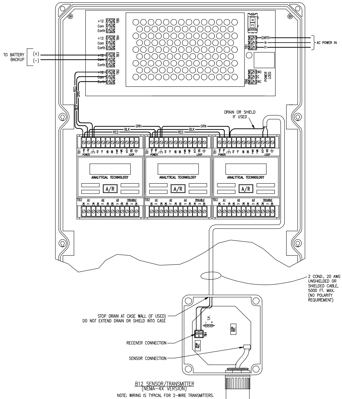
Figure 8: Receiver connection to 65W Power Supply (ATI-0545)
